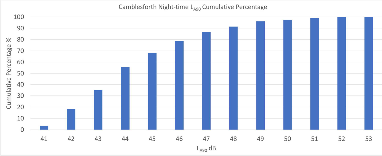
Plate 3.4 - Camblesforth 2020 Night-time Cumulative Percentage
