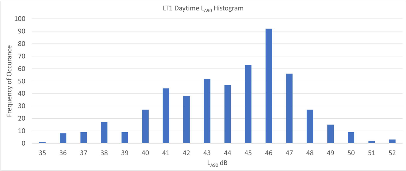
Plate 1.1 - LT1 Daytime Histogram
