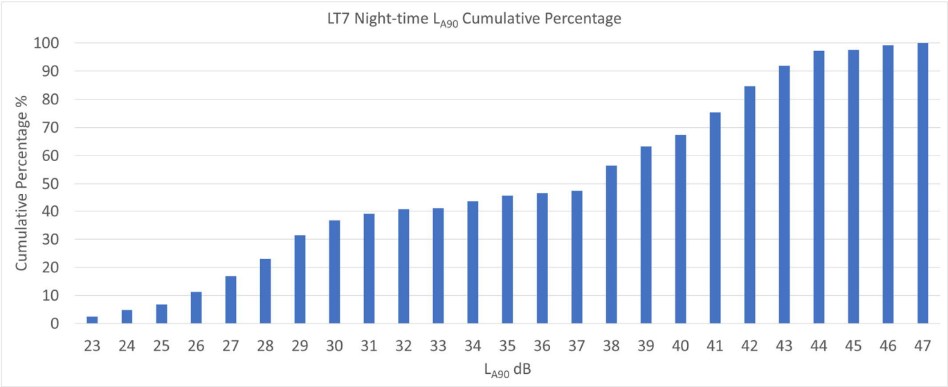
Plate 1.28 - LT7 Night-time Cumulative Percentage
