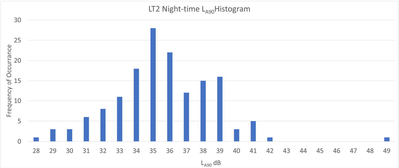
Plate 1.17 - LT2 Night-time Histogram
