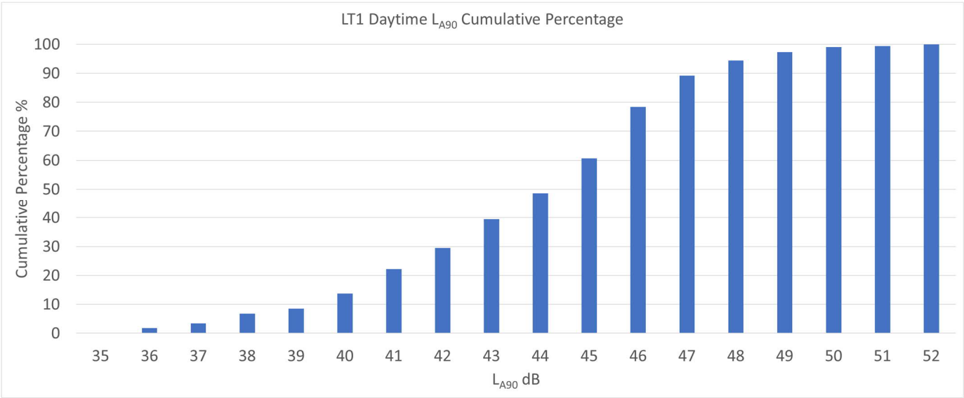
Plate 1.2 - LT1 Daytime Cumulative Percentage
