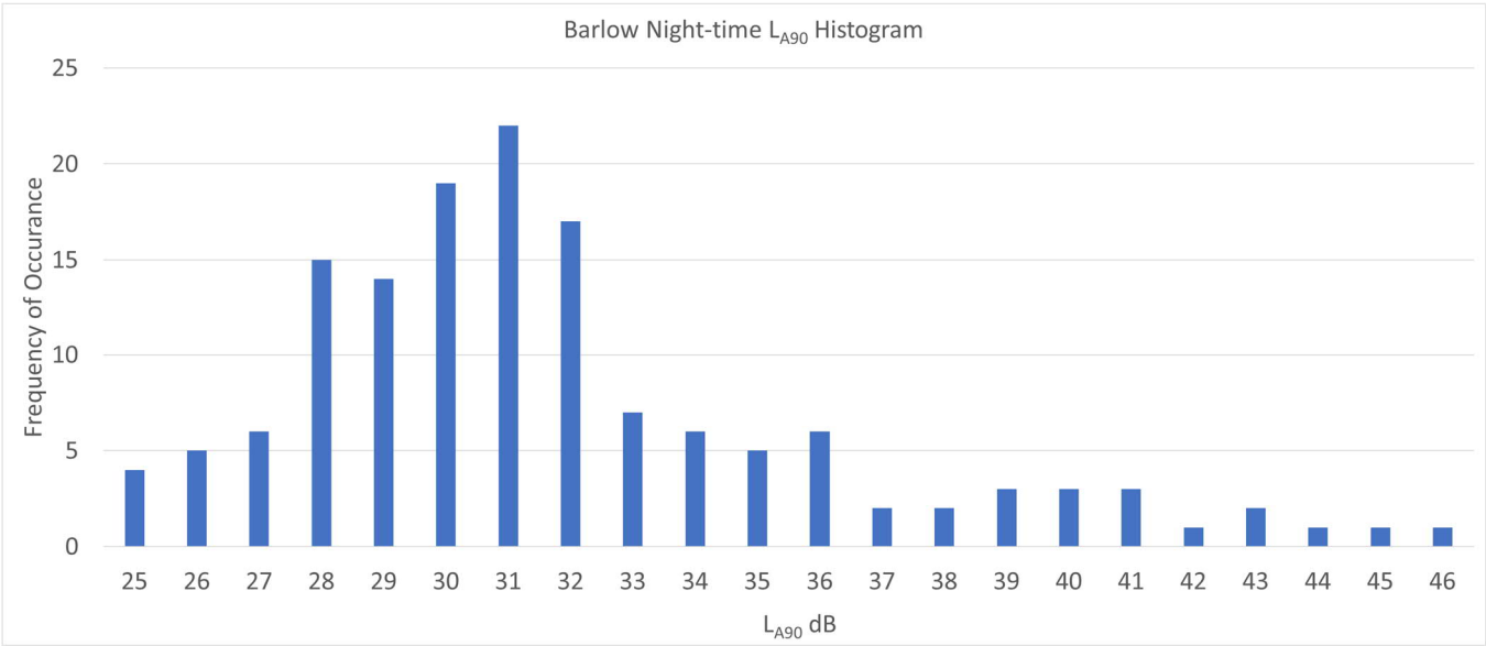
Plate 2.5 - Barlow 2021 Night-time Histogram
